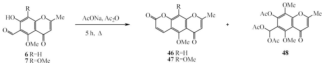
Scheme 17. Synthesis of pyrano[3,2- g ]chromene-2,6-diones ( 46 , 47 ) via the Perkin reaction
